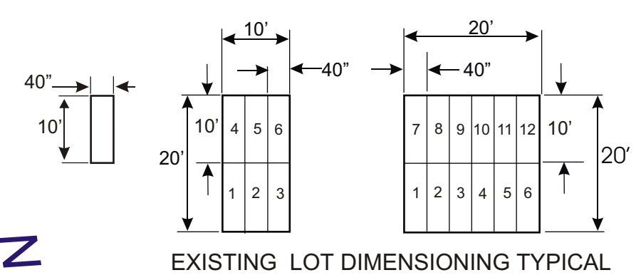
EXISTING LOT DIMENSIONING TYPICAL
