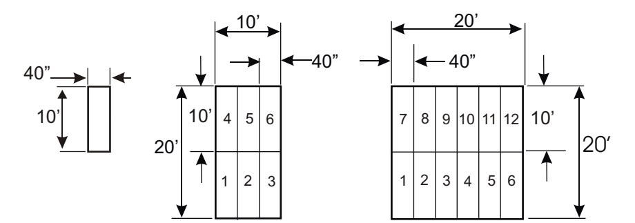
EXISTING LOT DIMENSIONING TYPICAL
